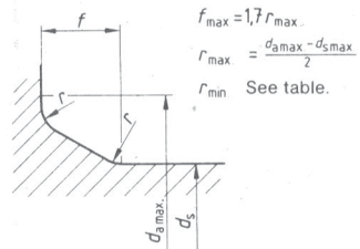
Detail X Maximum underhead fillet
