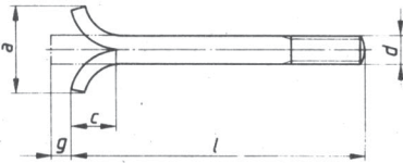
Type C, hot formed
