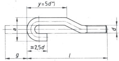
Type B (from M 16)
