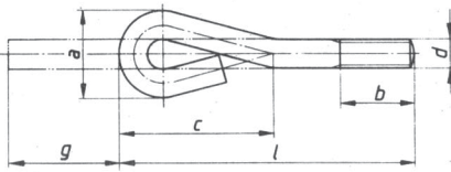
Type C, hot formed
