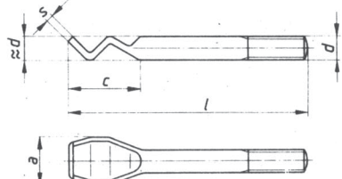
Type F (up to M 48)
