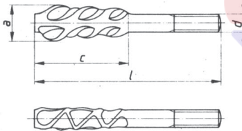
Type E (up to M 48)
